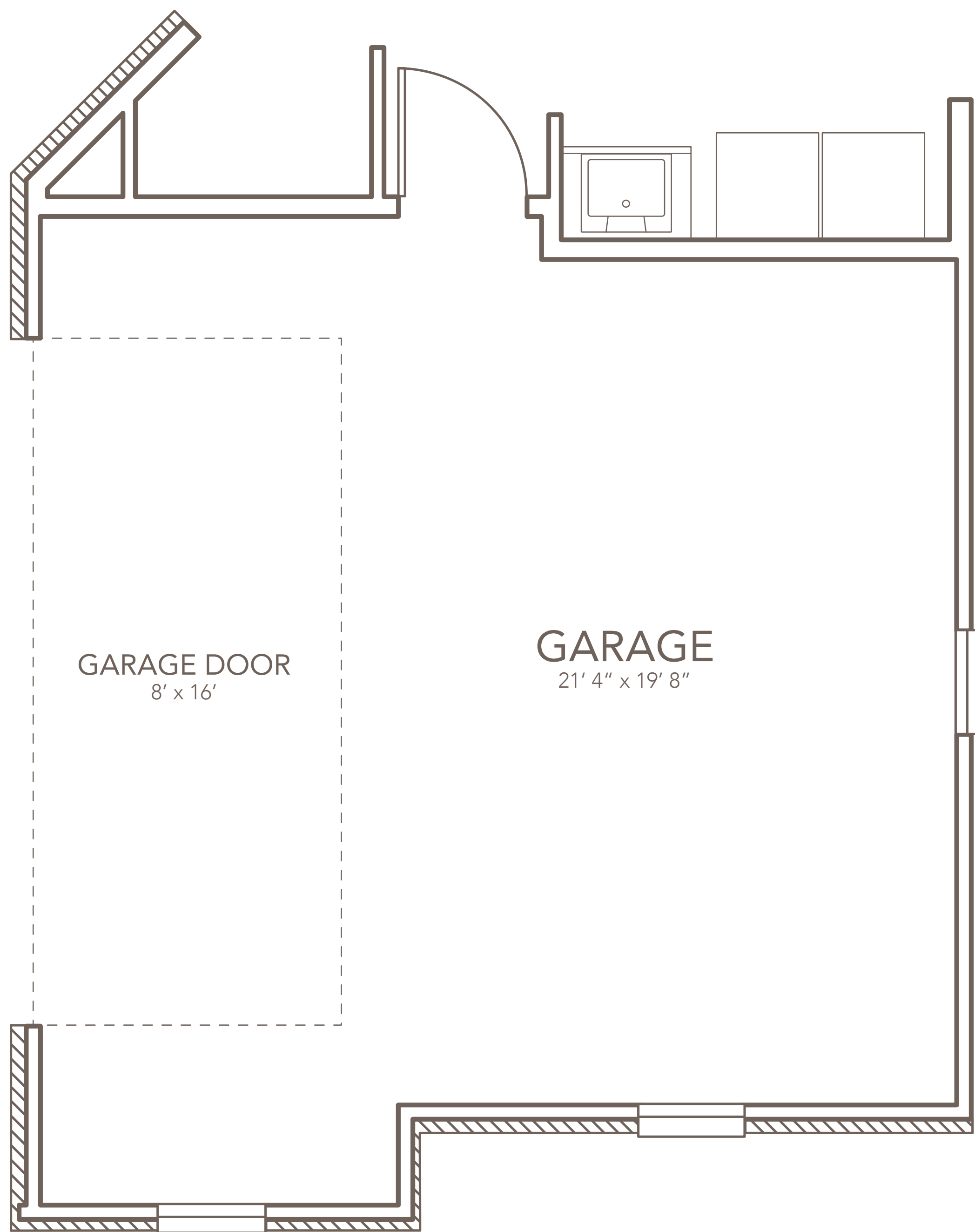
3 CAR GARAGE SIDE ENTRY
