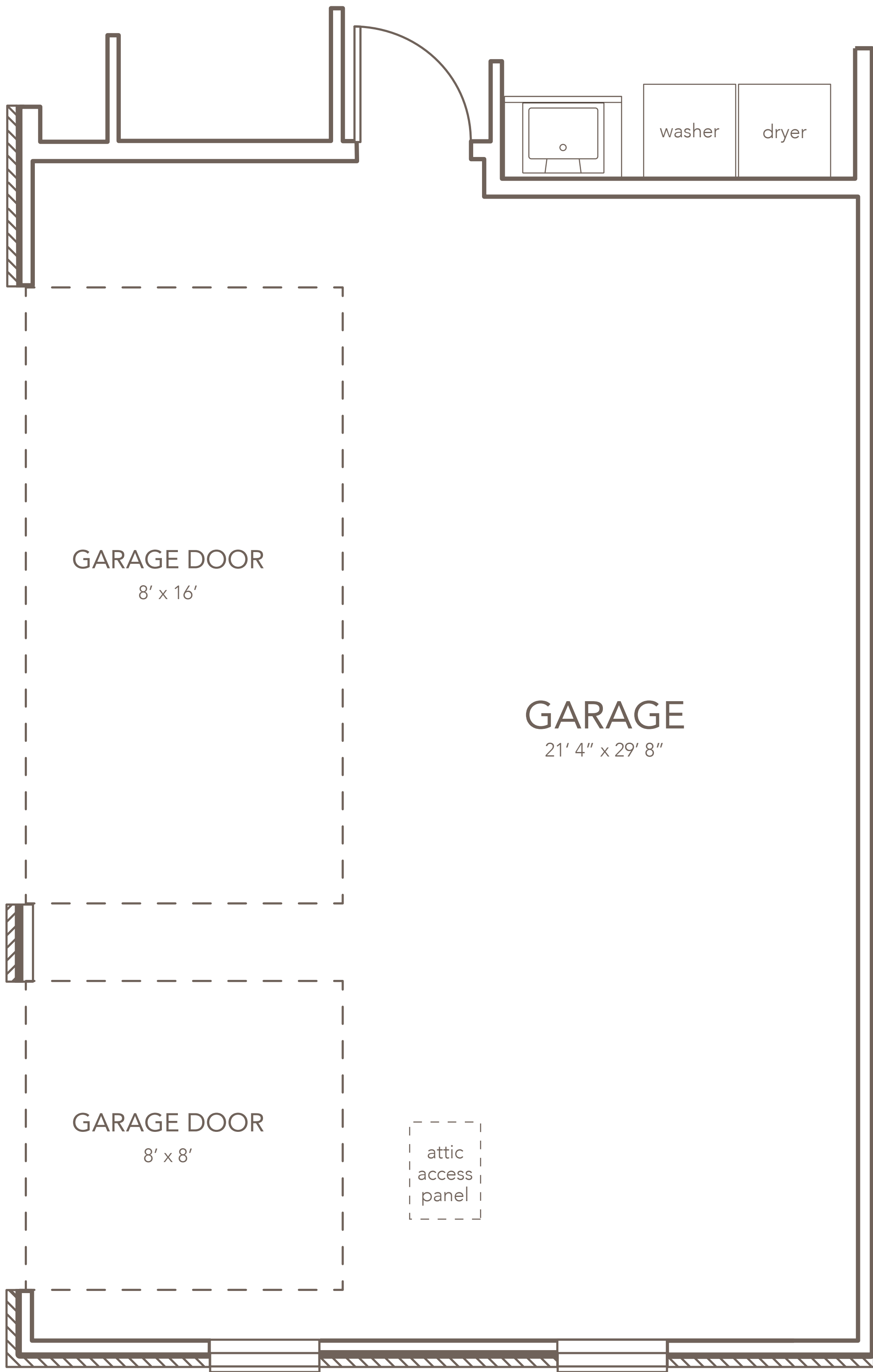
3 CAR GARAGE SIDE ENTRY
